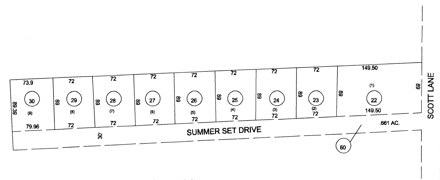
SUMMER SET DRIVE SUBDIVISION SCALE: 1"=100' INSET NO. 1
