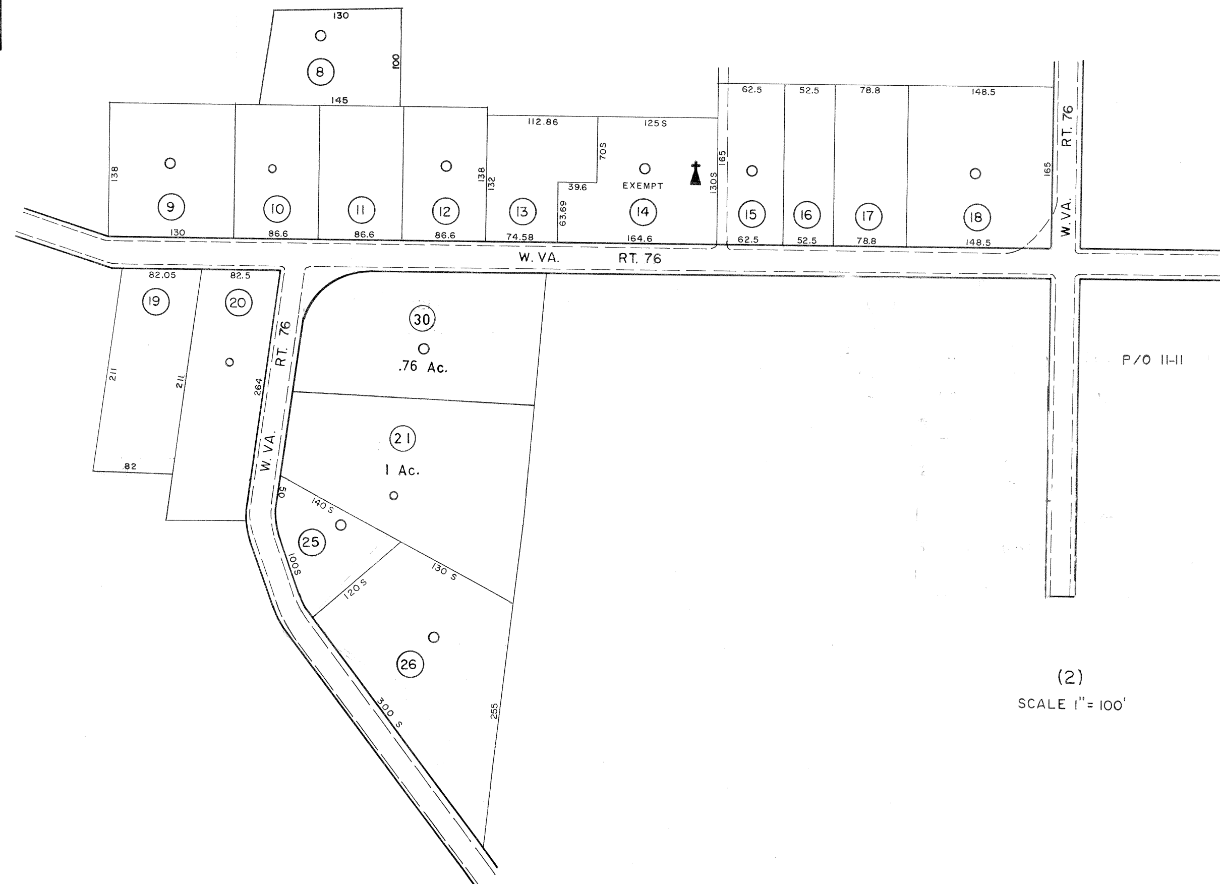
(1) SCALE 1" = 200'
